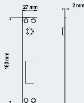
FLUSH MOUNTING TYPE
