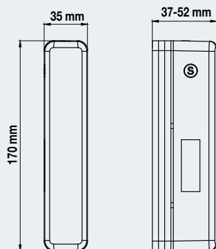
SURFACE MOUNTING TYPE
