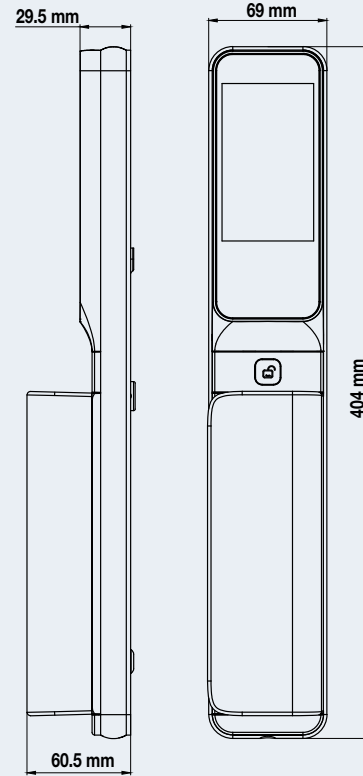
INDOOR UNIT
