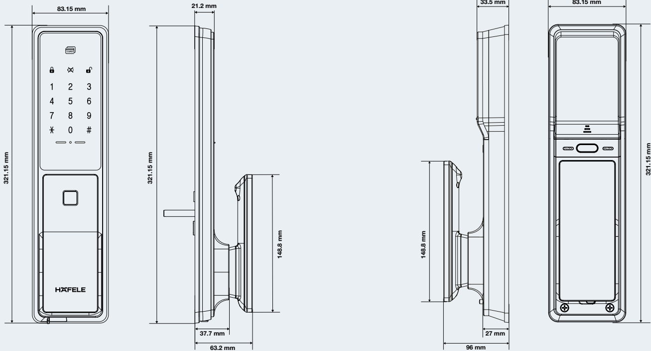
OUTDOOR UNIT
