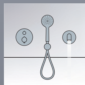
Thermostatic bath mixer for hand shower and separate bath spout
