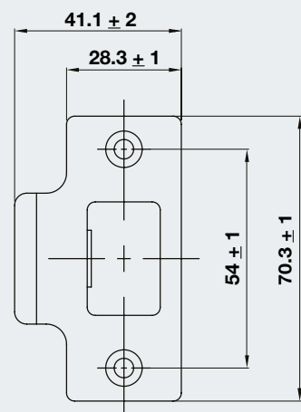
STRIKE PLATE SET
